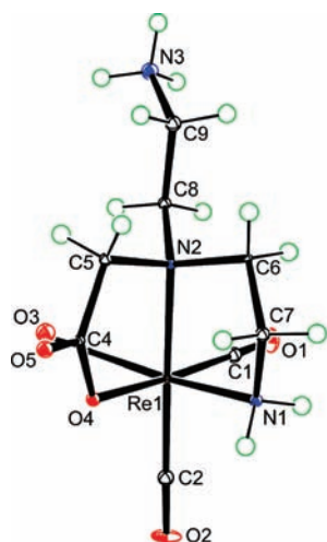
Figure 1. Perspective drawings of the complex in [\text{Re}(\text{CO})_3(\text{DTGH})\text{-NNO}]\text{PF}_6 \cdot \text{H}_2\text{O} ( 5 \text{PF}_6 \cdot \text{H}_2\text{O} ) (left) and [\text{Re}(\text{CO})_3(\text{DTG})\text{-NNN}] \cdot \text{H}_2\text{O} ( 6 \cdot \text{H}_2\text{O} ) (right) with 50% probability for the thermal ellipsoids. The \text{PF}_6^- anion and \text{H}_2\text{O} molecule are omitted for clarity.
