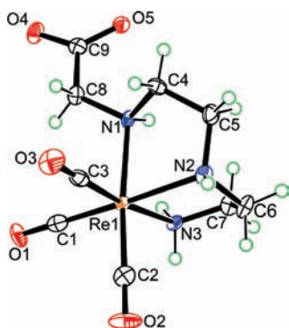
Figure 4. Perspective drawing of the complex in [\text{Re}(\text{CO})_3(\text{DTA})\text{-NNN}] \cdot \text{CH}_3\text{OH} ( 12 \cdot \text{CH}_3\text{OH} ) with 50% probability for the thermal ellipsoids. The methanol molecule is omitted for clarity.
