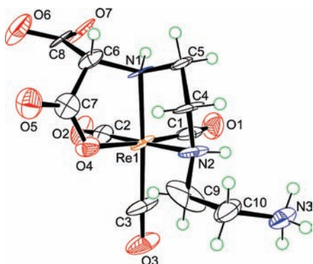
Figure 3. Perspective drawing of the complex in [\text{Re}(\text{CO})_3(\text{DTMH})\text{-NNO}] \cdot 2\text{H}_2\text{O} ( 9 \cdot 2\text{H}_2\text{O} ) with 50% probability for the thermal ellipsoids. The \text{H}_2\text{O} molecules are omitted for clarity.
